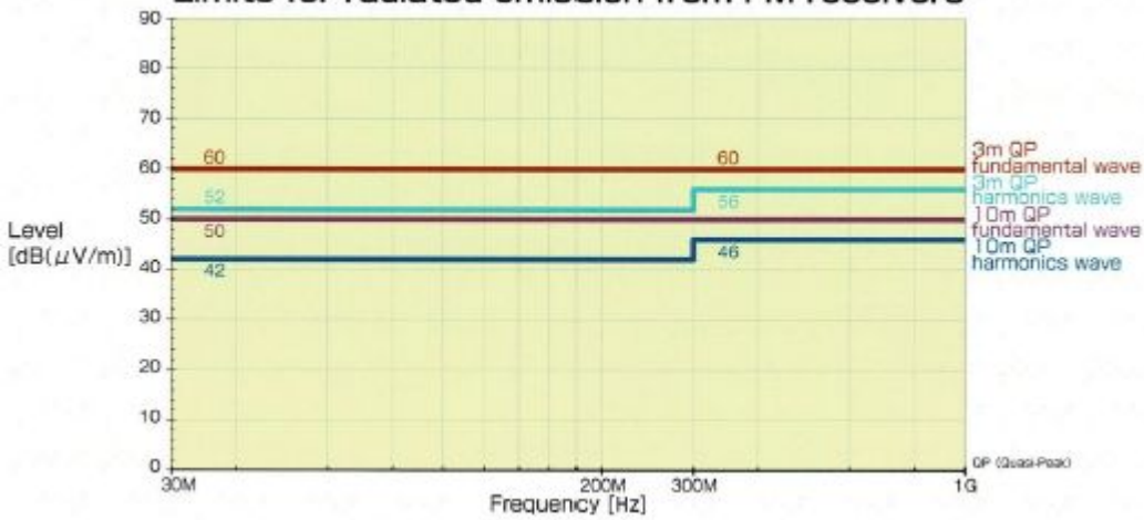
Limits for radiated emission from FM receivers
