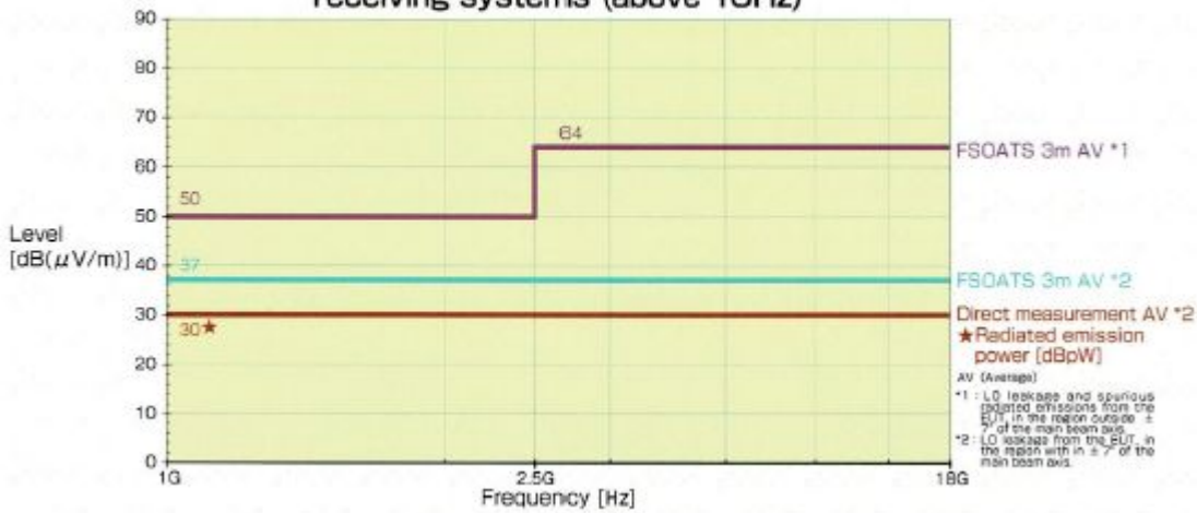
Limits for radiated emissions of outdoor units of home satellite receiving systems (above 1GHz)
